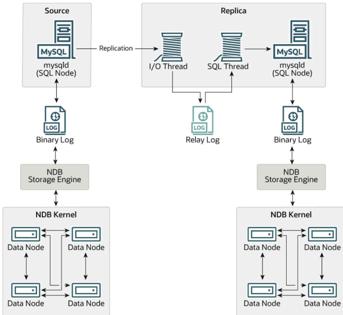
Figure 21.12 NDB Cluster-to-Cluster Replication Layout
