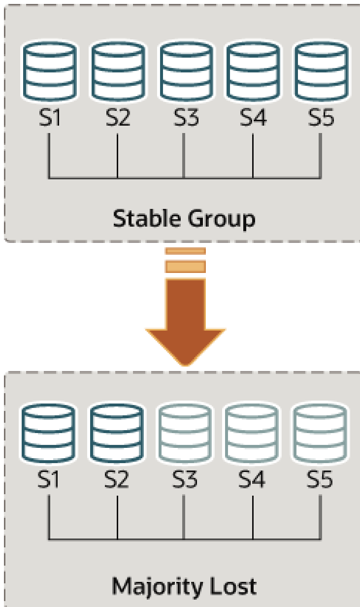
Figure 17.7 Losing Quorum
