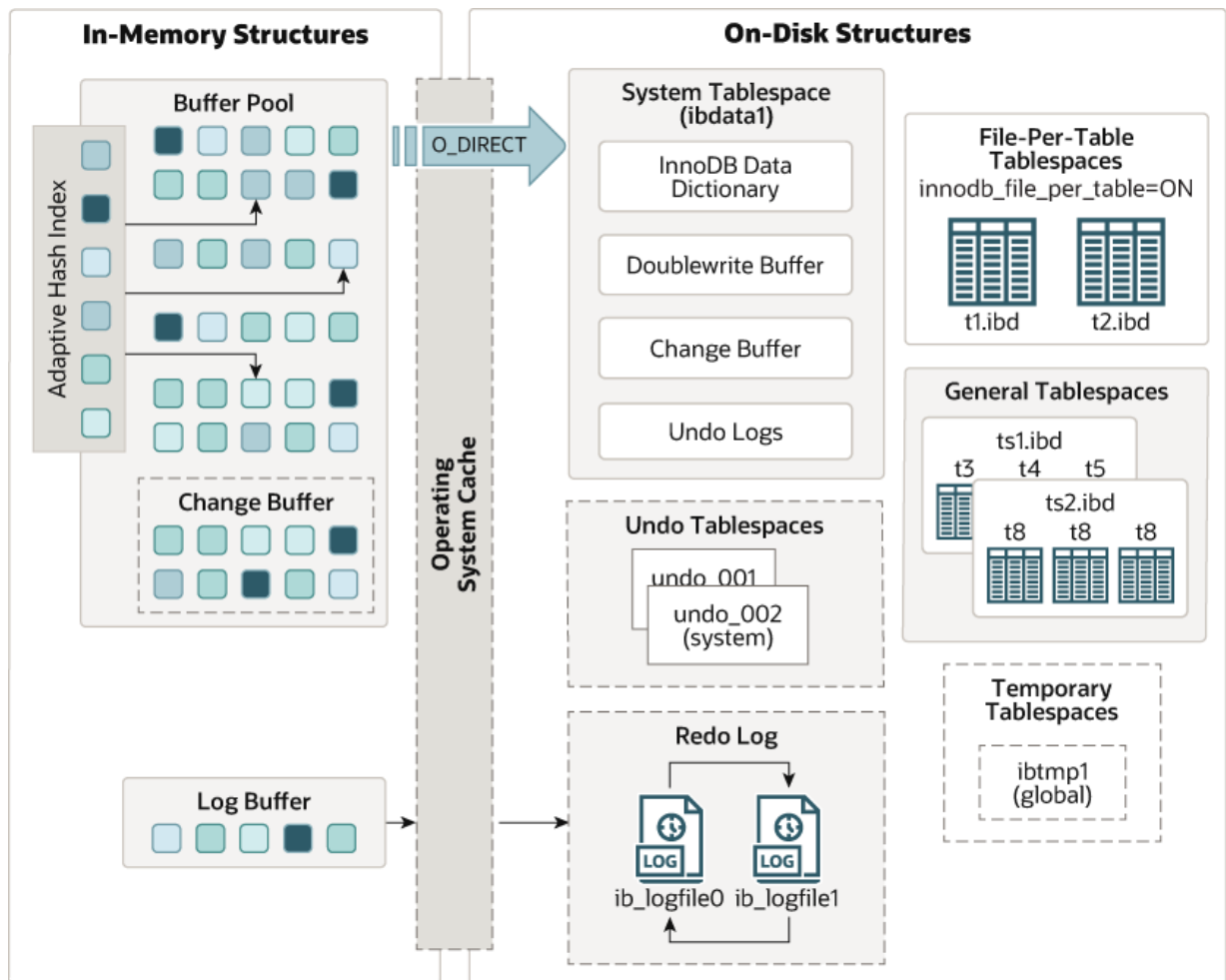
Figure 14.1 InnoDB Architecture
