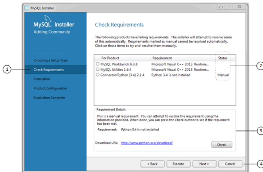
Figure 2.8 Check Requirements
