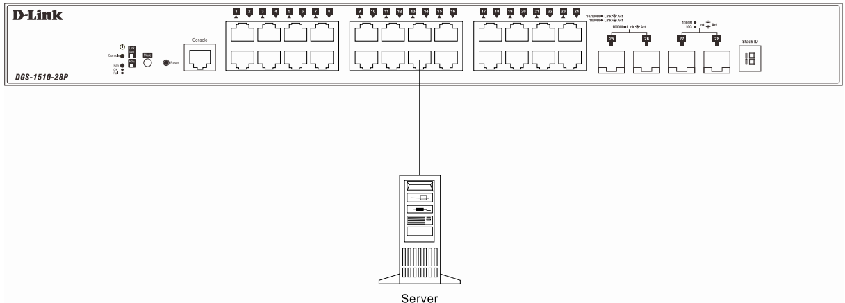
Figure 3-3 Server to Switch Connection
