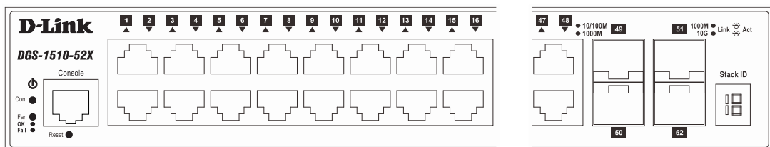
Figure 1-14 LED indicators for a DGS-1510-52X Switch
