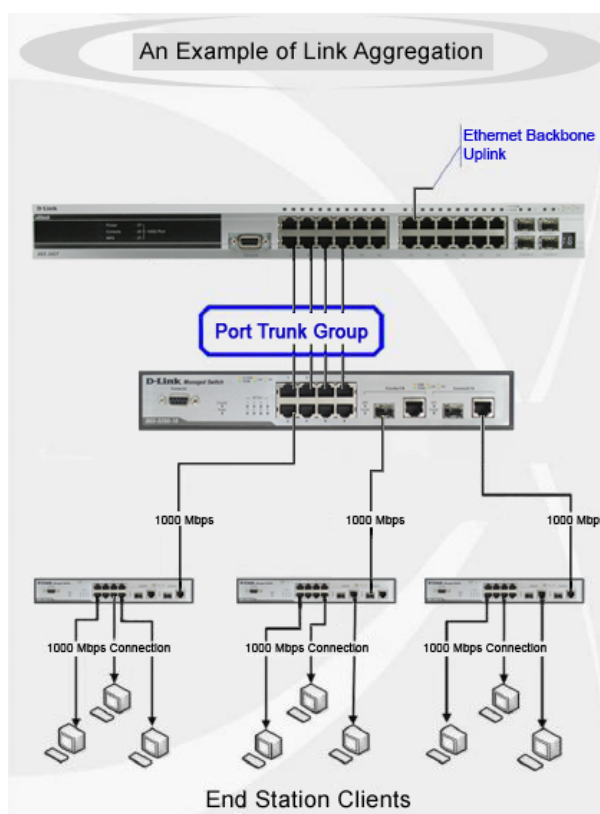
Figure 5-49 Example of Port Trunk Group
