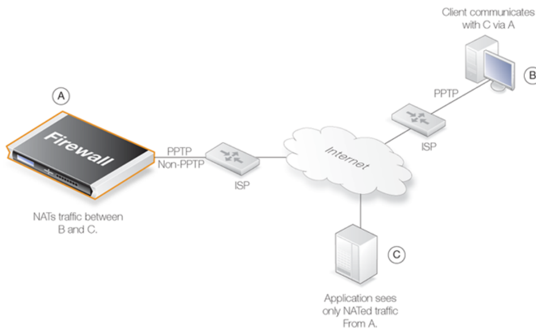
Figure 8.3. Anonymizing with NAT
