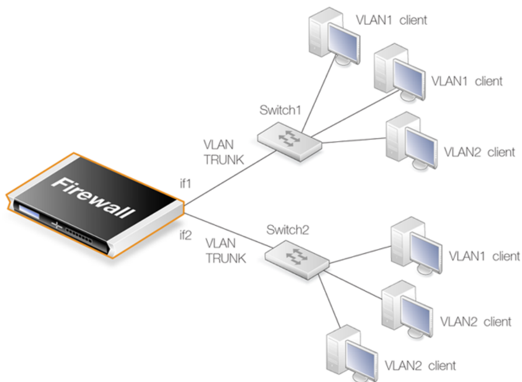
Figure 3.3. VLAN Connections
