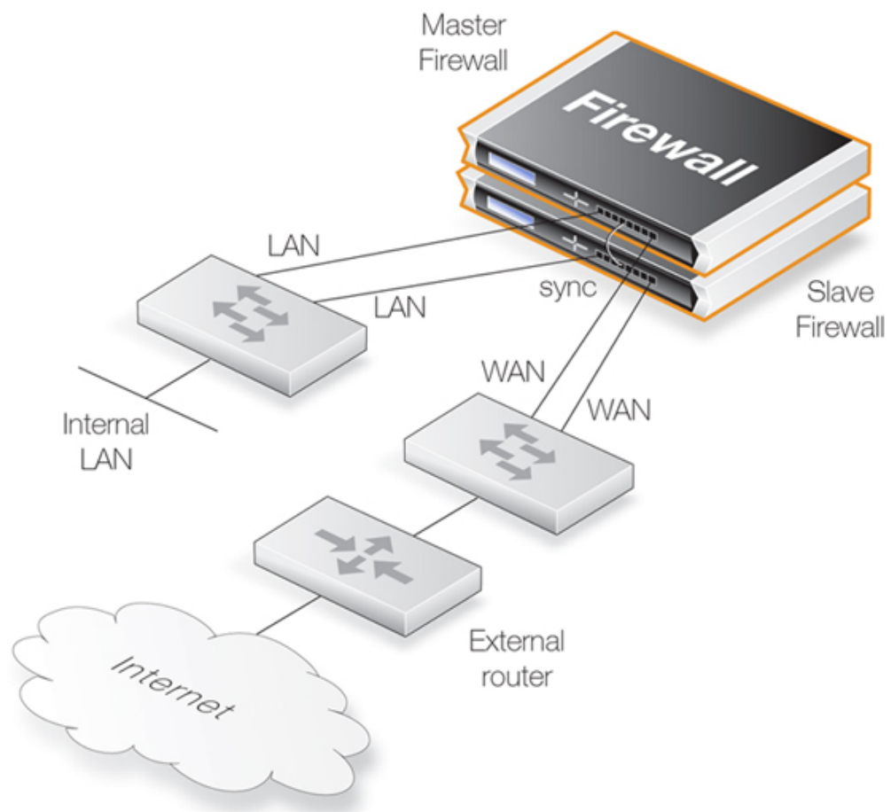
Figure 12.1. High Availability Setup
