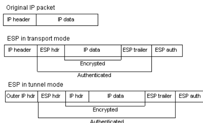
Figure 10.2. The ESP protocol
