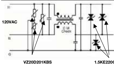
MOV In AC Line Protection
