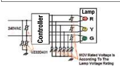
MOV In Traffic Light Protection
