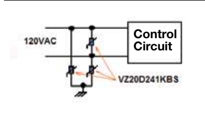
MOV In Control Circuit Protection
