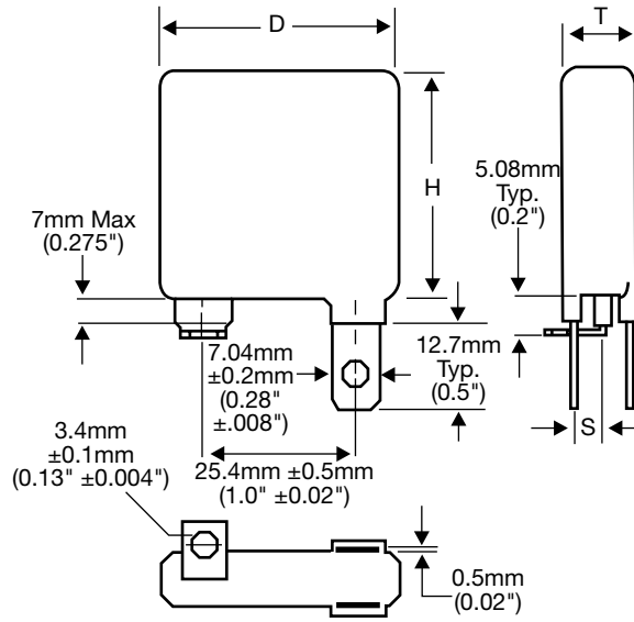
90° Bend Leads Part Number Suffix “KDQ”
