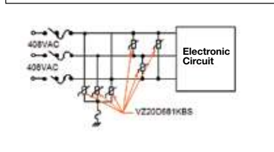
MOV for 3 Phase AC Line Protection
