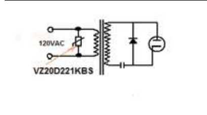
MOV In Microwave Oven
