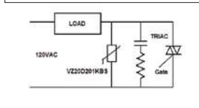
MOV in Triac Protection
