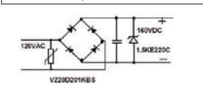
MOV in Bridge Rectifier Protection
