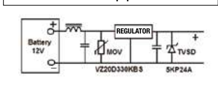
MOV in Automotive Equipment Protection
