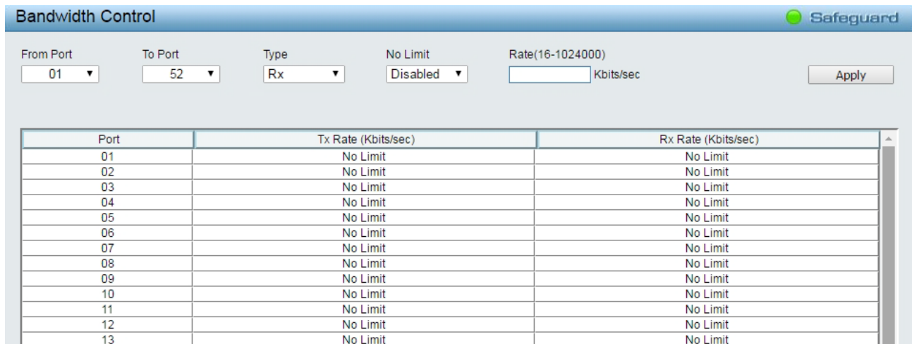
Figure 4.107 – QoS > Bandwidth Control
