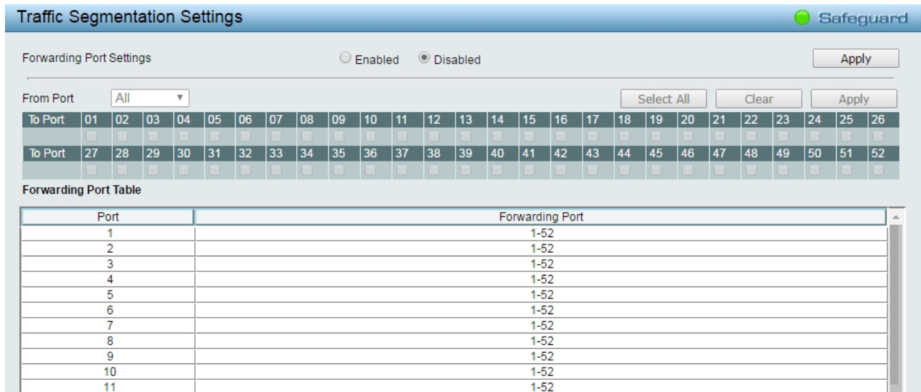
Figure 4.111 – Security > Traffic Segmentation
