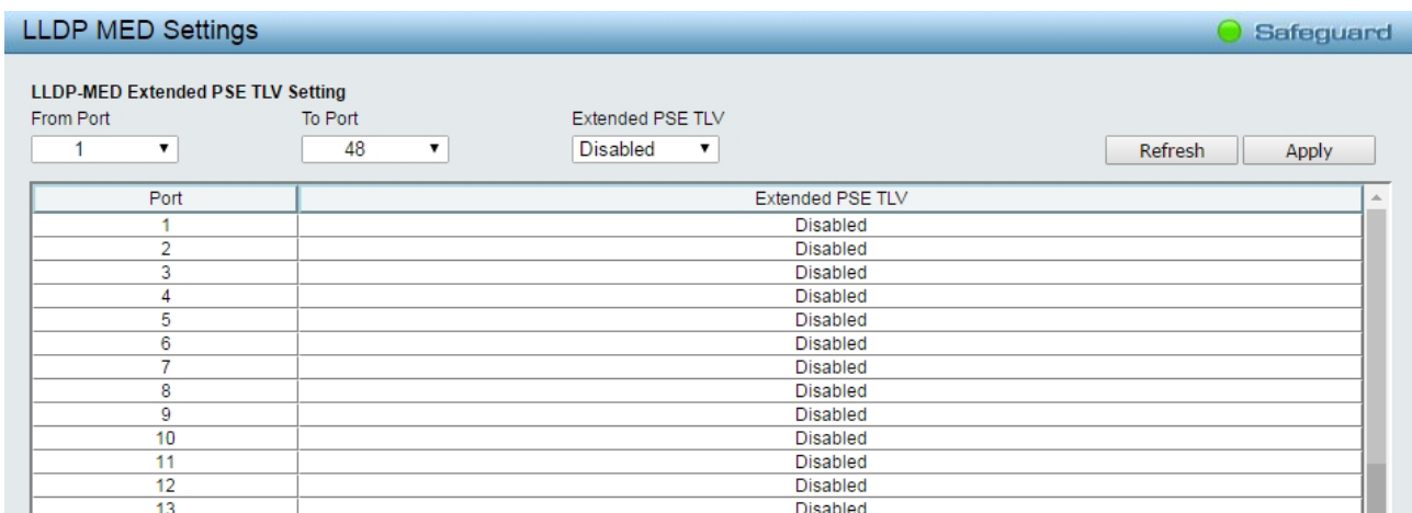
Figure 4.82 – L2 Functions > LLDP > LLDP-MED Settings
