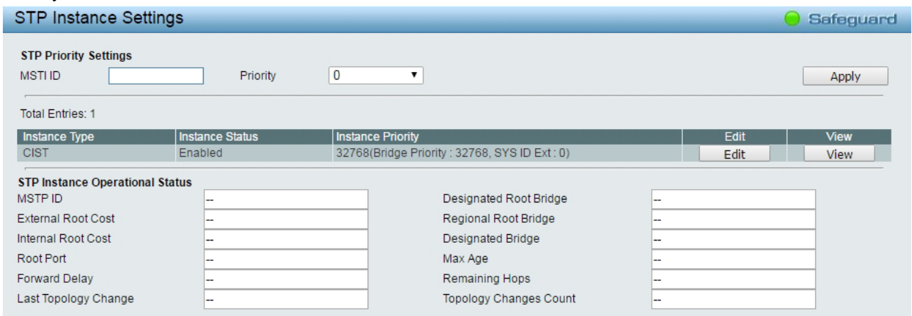
Figure 4.68 – L2 Functions > Spanning Tree > STP Instance Settings
