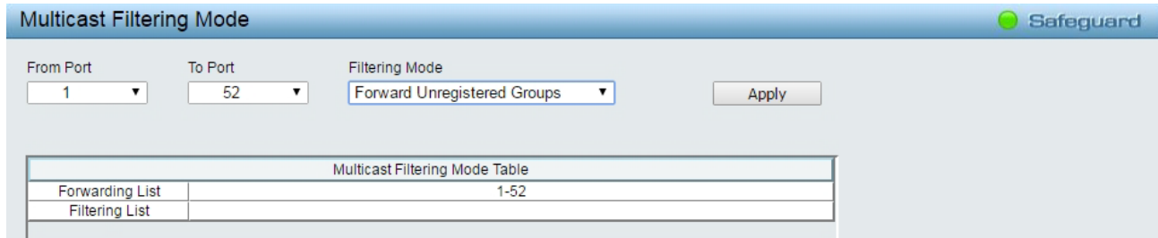
Figure 4.78 – L2 Functions > Multicast > Multicast Filtering Mode
