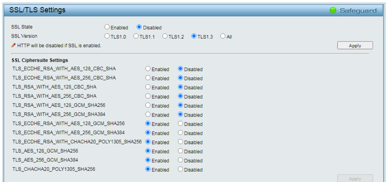
Figure 4.116 – Security > SSL/TLS
