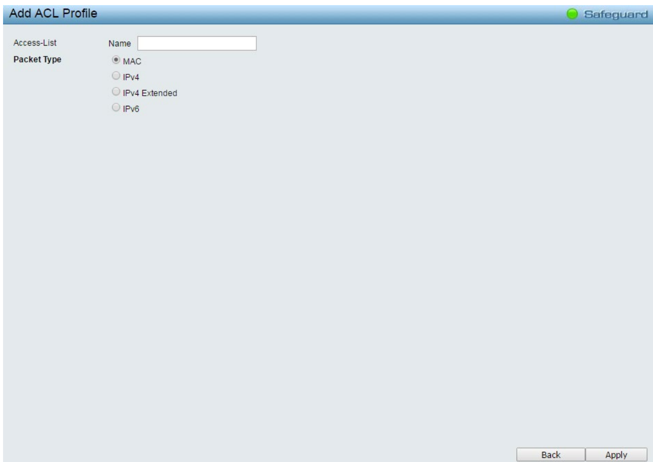
Figure 4.147 - ACL > ACL Access List – Add ACL Profile
